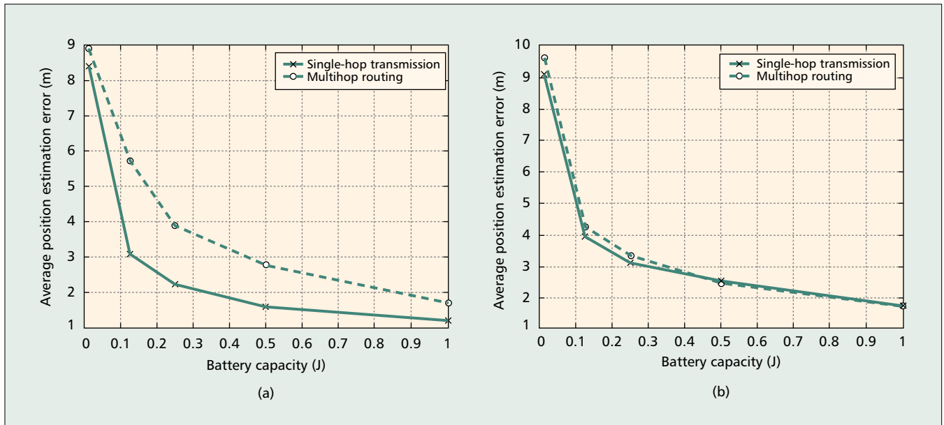
■ Figure 10. Performance comparison of different algorithms with different drop areas: a) 1 \text{ km} \times 1 \text{ km} ; b) 2 \text{ km} \times 2 \text{ km} .
