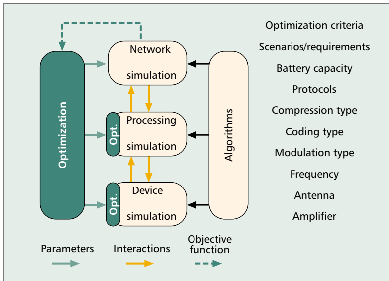
■ Figure 2. Layered design/optimization.
