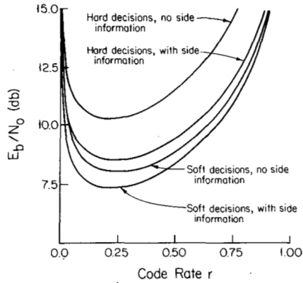
Fig. 3. E_b/N_0 needed for reliable communication for Rayleigh fading with and without side information available (hard and soft decisions).
